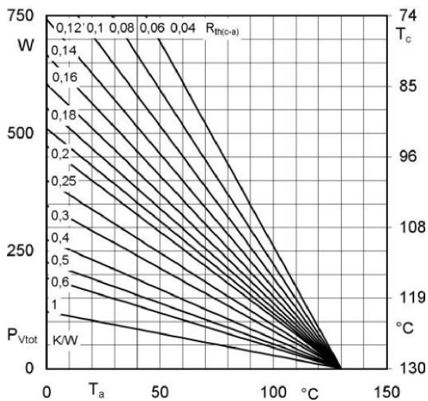
Power loss of two module vs case temperature
