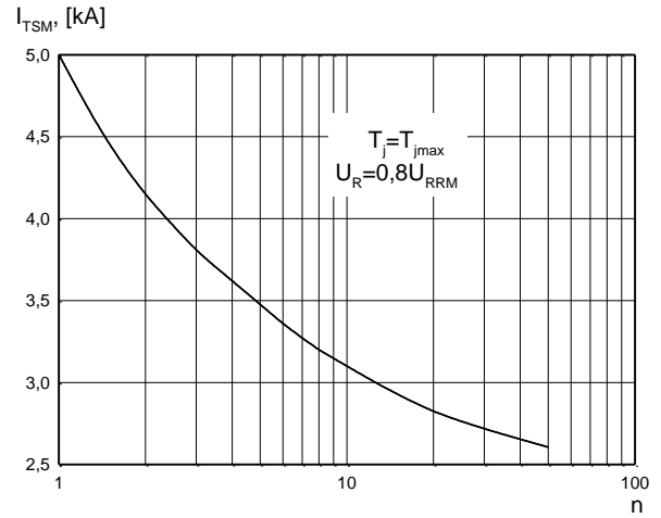
Non-repetitive surge current rating
